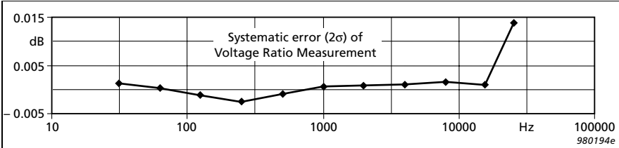
Fig. 7. Systematic error of Voltage Ratio measurement. The error is measured by using an electrical reference standard which is developed by National Physical Laboratory (UK). The result is obtained with a system similar to Type 9699 used by DPLA (explained later)
